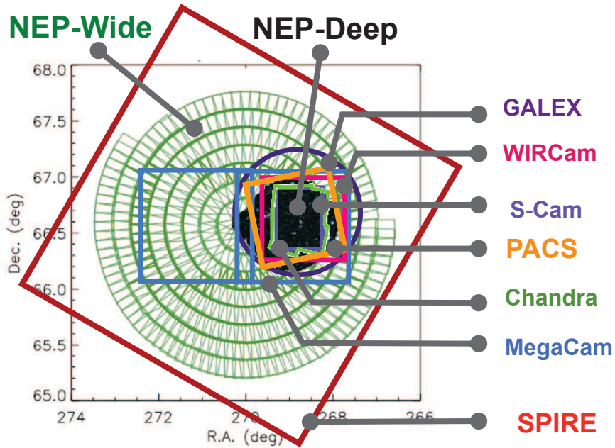
Figure 1 Sky coverage of the multi-wavelength data around NEP. See Table 1 for more information (e.g. areas, depths). Ne
