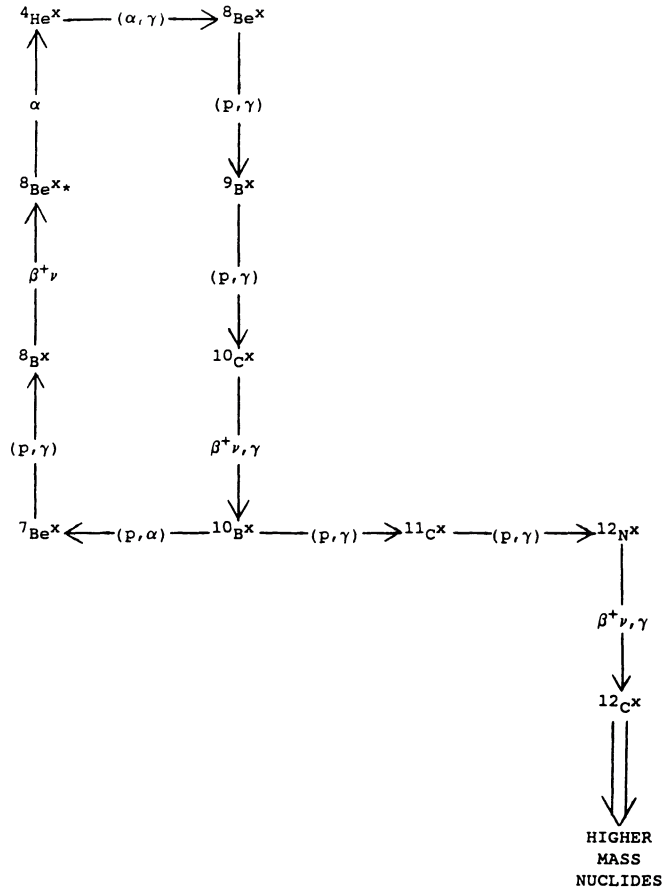
FIG. 1.—Energy-generating cycle via hydrogen burning of X^- nuclides. Note that {}^8\text{Be}^x is stable, making possible the high efficiency of this cycle.
