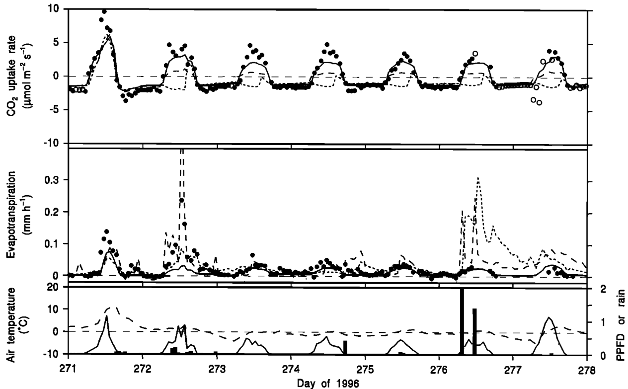
Figure 4. Same as Figure 2, except for days of the year 271–277, 1996.
