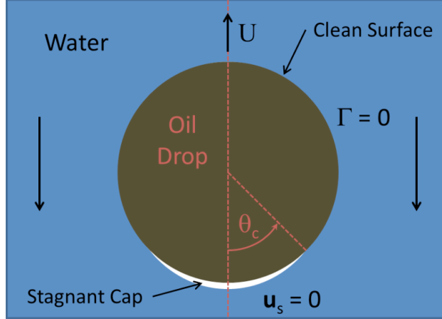
Figure 5.2: A surfactant-laden drop rising in a uniform ambient, with negligible surface diffusion. The surfactant appears in white as a cap on the bottom of the drop, which transitions to a clean surface at a cap angle, \theta_c .
