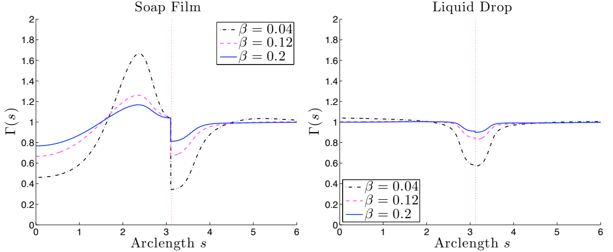
Figure 4.14: Surfactant profile redistributed by gravity at the time of maximum deformation for a soap film (left) and a liquid drop (right) The vertical line shows the point where merging begins - so that the portion of the plot to the left of the vertical line describes the drop, and the portion of the plot to the right describes the reservoir.
