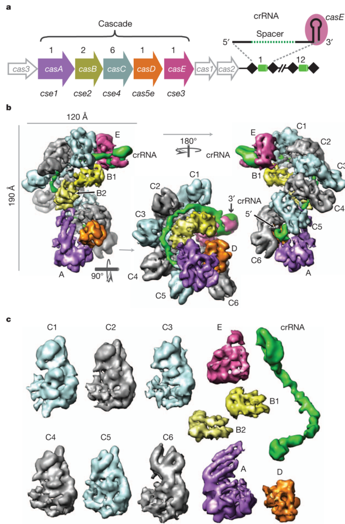
Figure 1. Structure of the Cascade complex from E. coli
