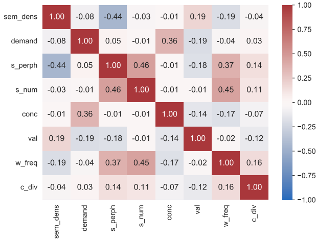
Figure 2: Heatmap of Pearson correlations for each factor, using differences between every pair of senses.
