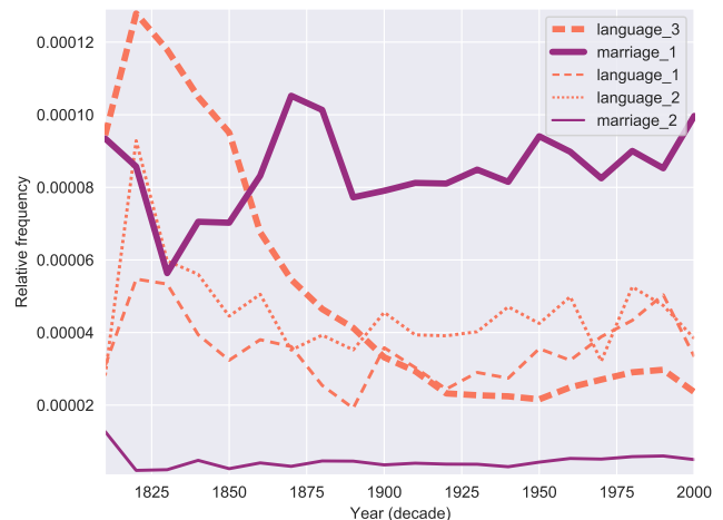
Figure 1: An illustration of a declining and stable pair of senses in our study: language_3 (“style of writing or speech”) and marriage_1 (“formal union of two partners in a personal relationship”). Thinner lines with the same colour are other senses of the same word. These include: language_1 (“the method of human communication”), language_2 (“a communication system used by a particular community”), and marriage_2 (“a mixture of elements”).
