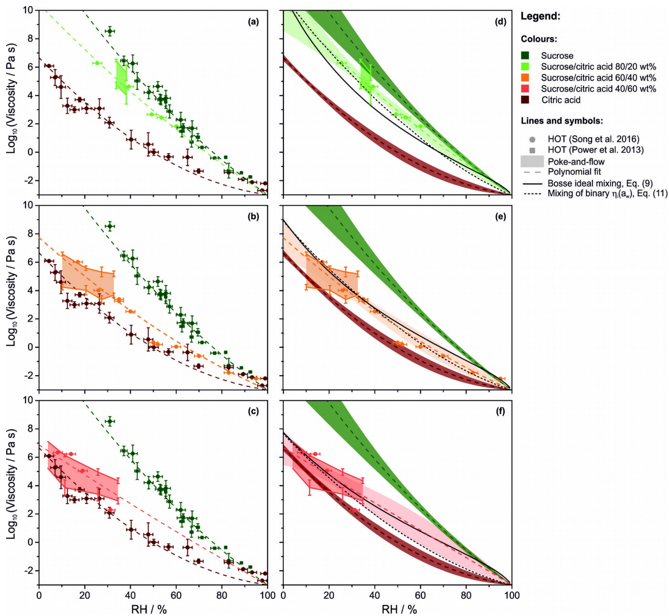
Figure 3. Measured and modelled relative humidity-dependent viscosity of sucrose/citric acid mixtures (80/20 wt%, panels a-d; 60/40 wt%, panels b-e; 40/60 wt%, panels c-f). Data for binary sucrose 26,28 and citric acid 26 are also reported for comparison. Symbols: circles – HOT data (60/40 wt% mixture in panels b and e from previous work); 31 solid lines – poke-and-flow measured upper and lower limits of viscosity (shaded area included to guide the eye); dashed lines – 2 nd order polynomial fit of HOT and poke-and-flow data (the envelopes in panels d, e and f represent the 95% confidence bands of the fitting); 31 solid line – prediction from Bosse ideal mixing (Eq. (9)); short dashed line – prediction from mixing of binary viscosity values (Eq. (11)). Colors: dark green – sucrose; light green – 80/20 wt% sucrose/citric acid mixture; orange – 60/40 wt% mixture; red – 40/60 wt% mixture; brown – citric acid.
