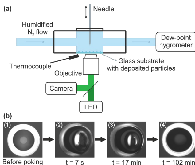
Figure 2. (a) Poke-and-flow experimental setup. (b) Images of an 80/20wt% sucrose/citric acid particle before (1) and after poking (2) - (4). Time after poking is indicated below the images in (2)-(4).
