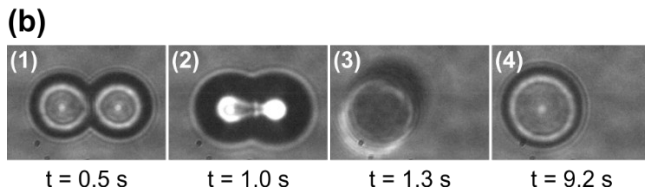
Figure 1. (a) Holographic Optical Tweezer (HOT) experimental setup. (b) Brightfield images of two coalescing droplets (sucrose/critic acid 60/40 wt% mixture, RH=39%). The aspect ratio is inferred for time-points at which the composite non-spherical particle is clearly situated in the image plane.
