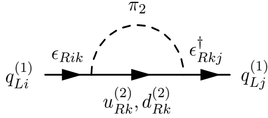
FIG. 4: Wavefunction renormalization that results in the flavor-dependent running of the parameter \epsilon_L in the effective theory valid in the energy range below the cutoff scale and above the masses of the heavy fermions. This running yields the renormalization group equation (62). Note that the q_L^{(1)} and u_R^{(2)}, d_R^{(2)} are the site 1 and 2 gauge-eigenstate fermion fields of Eq. (1). In 't-Hooft-Feynman gauge, the leading contribution comes from \pi_2 , the unphysical Nambu-Goldstone Boson in the non-linear sigma model field \Sigma_2 of Eq. (2).
