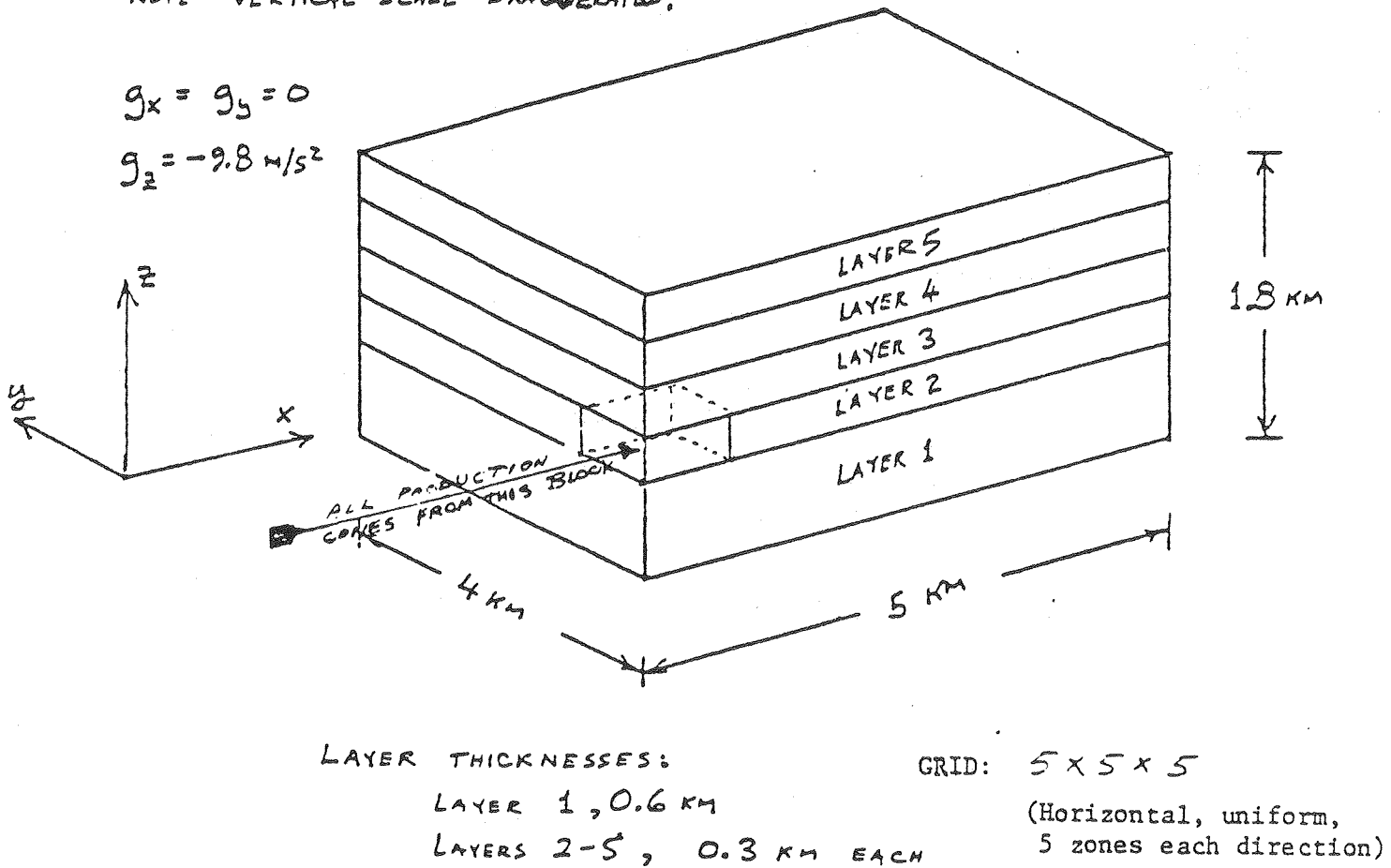
Figure 1: Geometry of the reservoir and mesh design.
