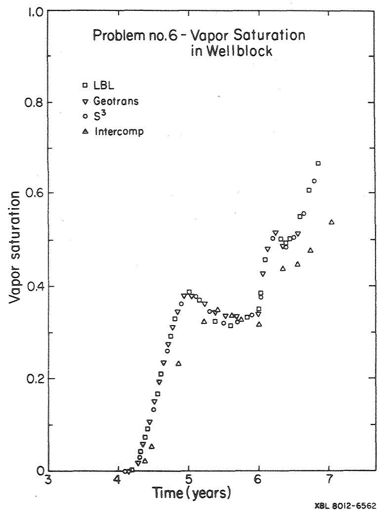
Figure 3: Evolution of vapor saturation in well block.
