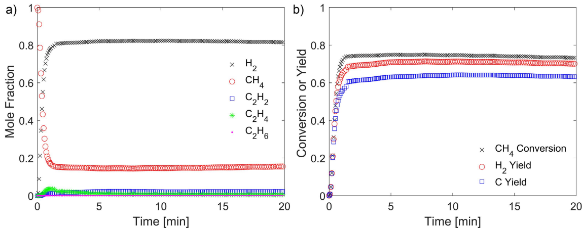
Figure 4.15: Real-time monitoring results from the calibrated mass spectrometer showing (a) mole fractions in the product stream, and (b) methane conversion and product yields for CH_4 decomposition through ceramic felt at 100 scfm flow rate, 3.33 kPa pressure, 1.86 kW solar power, and 20 min reaction period.
