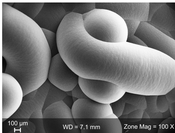
Figure 4.14: SEM image of the carbon felt's central region after \text{CH}_4 decomposition and carbon deposition at 100 sccm flow rate, 3.33 kPa pressure, 1.86 kW solar power, and 120 min reaction period.
