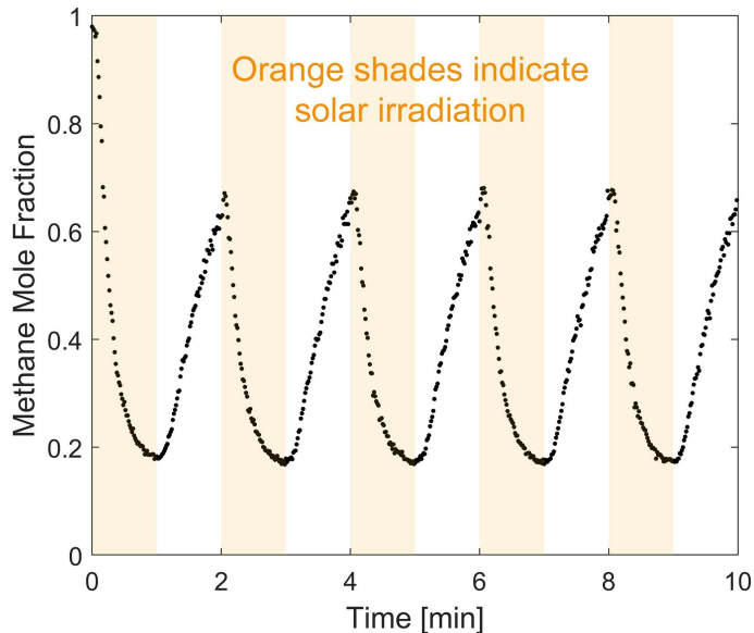
Figure 4.7: Methane product mole fraction as a function of time under HFSS solar irradiation cycling in an on/off manner at flow rate of 100 sccm, pressure of 3.33 kPa, solar power of 1.86 kW, and medium thickness of 3.2 mm.
