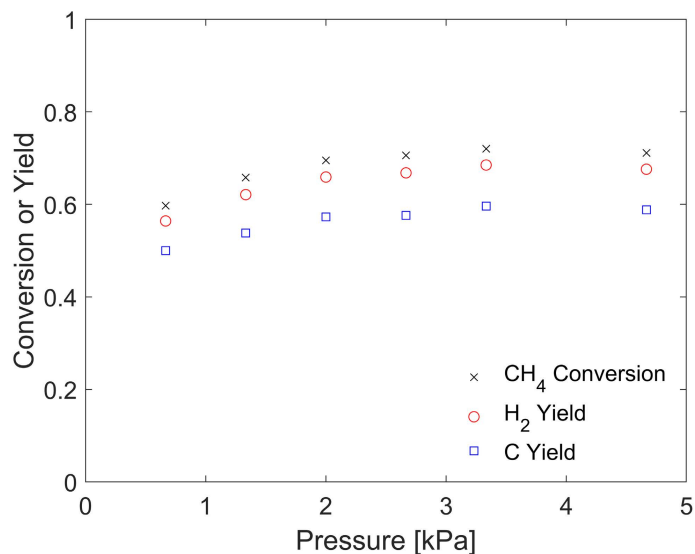
Figure 6.8: Effect of pressure on methane conversion and product yields for roll-to-roll methane pyrolysis at methane inlet flow rate of 100 sccm and solar power of 2.34 kW, with 0.89 mm thick roll.
