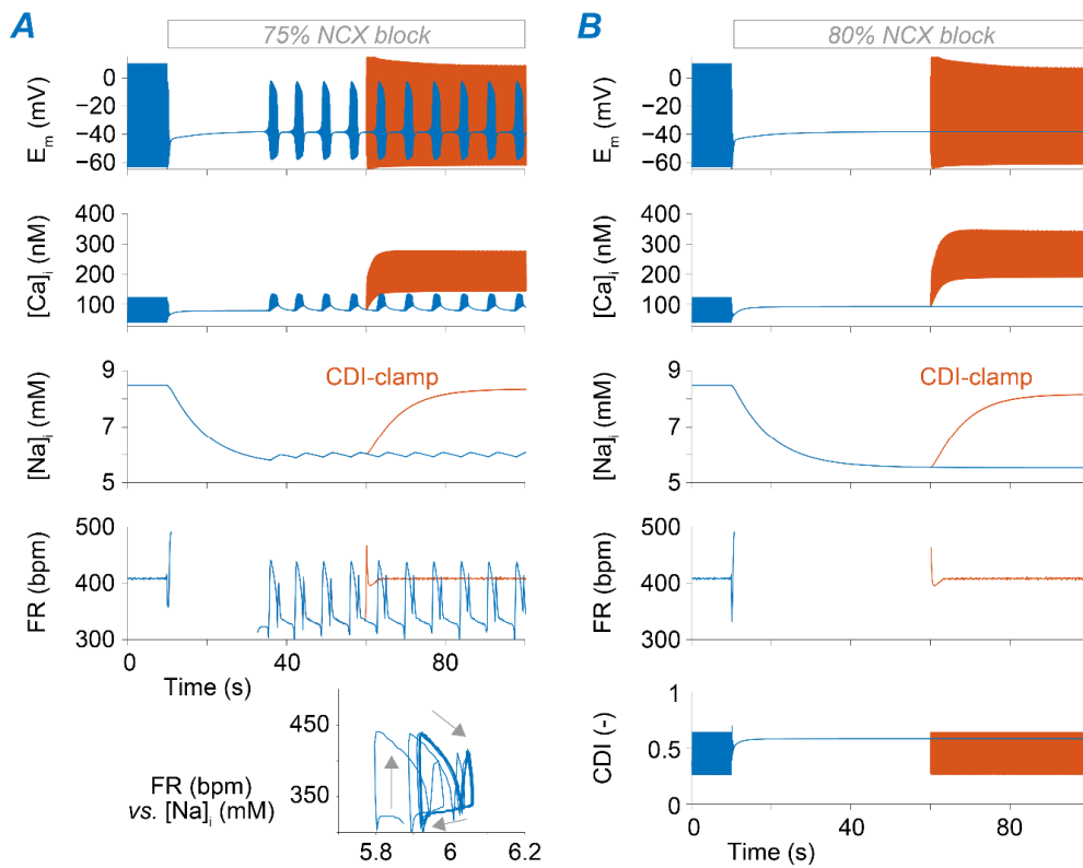
Figure 6. \text{Ca}^{2+} -dependent I_{\text{CaL}} inactivation upon NCX block impairs SAM automaticity. (A) Time course of membrane potential, [\text{Ca}^{2+}]_i , [\text{Na}^+]_i , and FR upon simulation of 75% block of NCX (at t = 10 s). The inset shows the FR- [\text{Na}^+]_i phase plot obtained when the model enters the bursting regime. (B) Time course of membrane potential, [\text{Ca}^{2+}]_i , [\text{Na}^+]_i , FR, and CDI of I_{\text{CaL}} upon simulation of 80% block of NCX (at t = 10 s). In both panels, orange traces are obtained by imposing (after t = 60 s) the values of CDI predicted before NCX block; blue traces are obtained simulating the model without any constrain on CDI.
