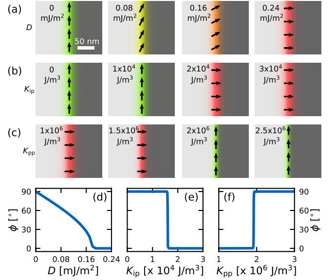
FIG. 2. Domain wall images as a function of (a) DMI constant D and (b) in-plane anisotropy constant K_{ip} for a perpendicular anisotropy constant K_{pp} = 1 \times 10^6 \text{ J/m}^3 . (c) Images as a function of K_{pp} for K_{ip} = 3 \times 10^4 \text{ J/m}^3 . Corresponding domain wall magnetization angles \phi as a function of (d) D , (e) K_{ip} , and (f) K_{pp} .
